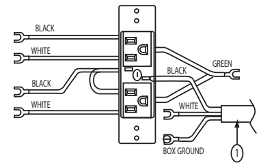
⑤ CIRCUIT BREAKER/OUTLETS ASSEMBLY
