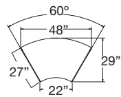
60° Curve
