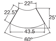
60° Curve
