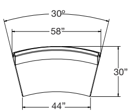
Double Seat, Uph 30° Inside Curve
