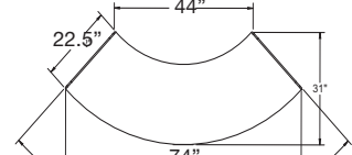
90° Curve
