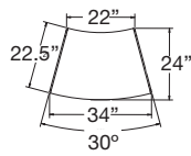
30° Curve
