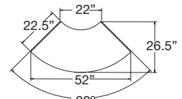
90° Curve
