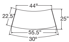
30° Curve
